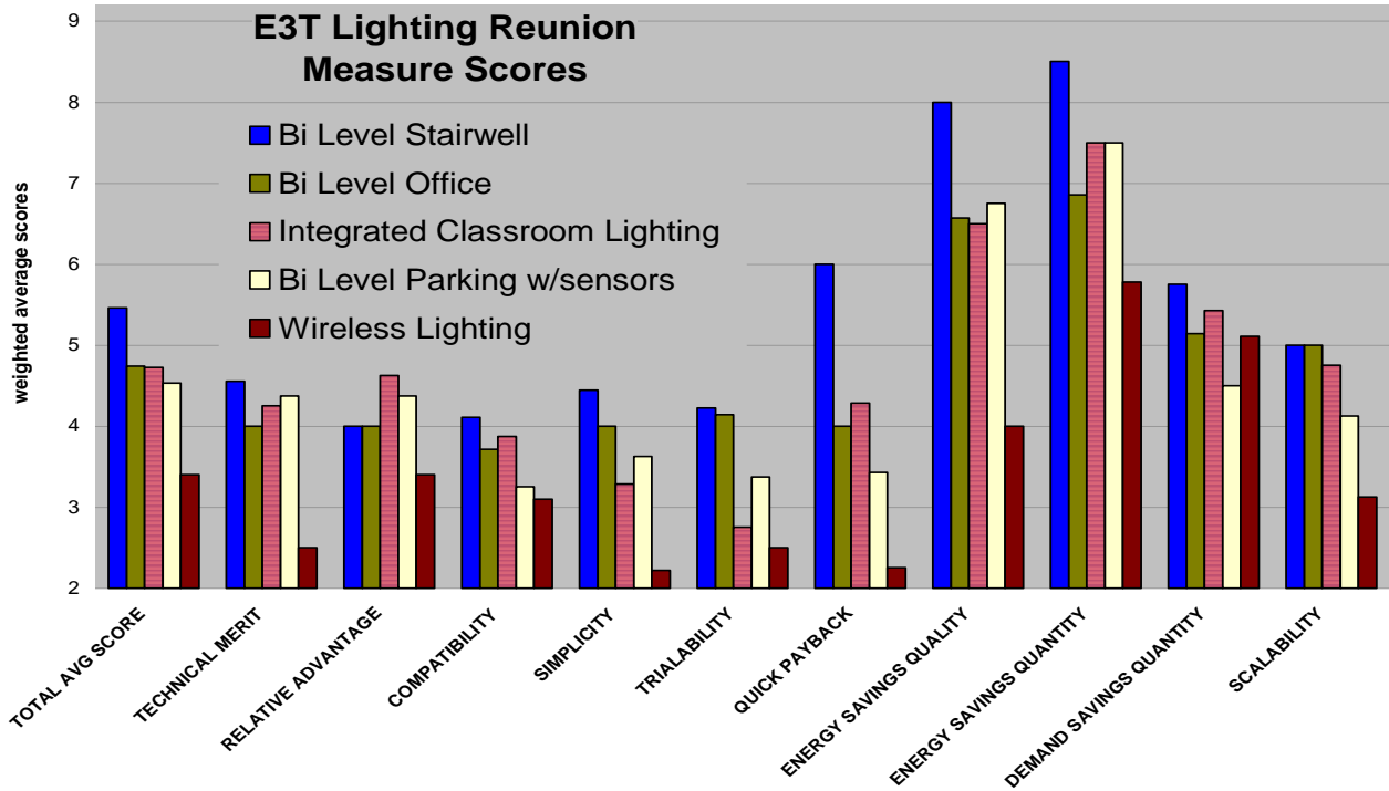
Figure 1. Graphical Representation of Measure Scoring
